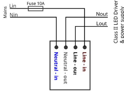
LED SPD 10kVIII T3 T3 type connections when "end of life" is reached the protector and load are switched off from mains
