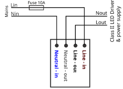
LED SPD T2&T3 10kVIII T3 type connections when "end of life" is reached the protector and load are switched off from mains
