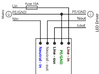
LED SPD 10kVL T3 T3 type connections when "end of life" is reached the protector and load are switched off from mains
